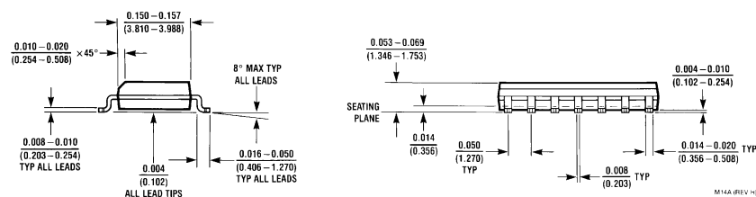
14-Lead Small Outline Molded Package (M) Order Number DM74LS132M NS Package Number M14A
